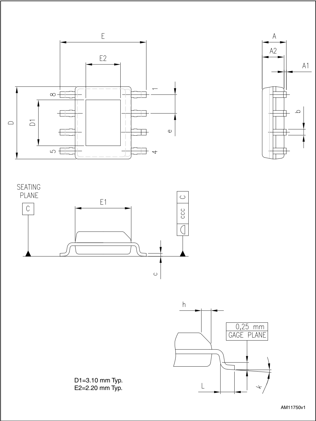
Figure 37. Package dimensions
