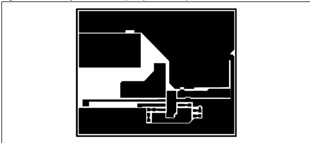
Figure 18. PCB layout: L7986TA (component side)
