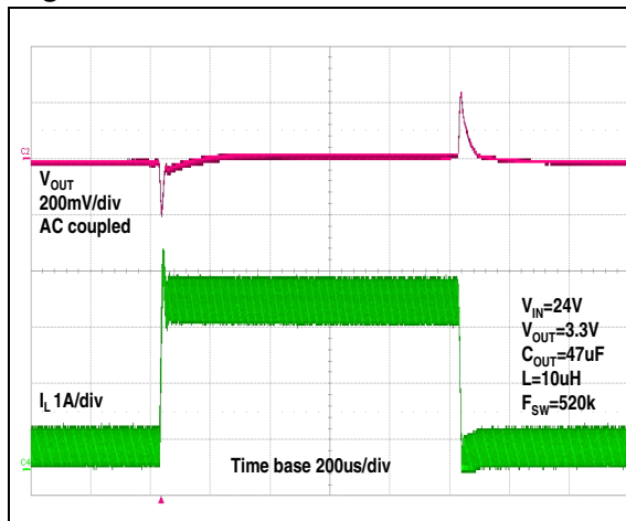
Figure 29. Load transient: from 0.4 A to 3 A
