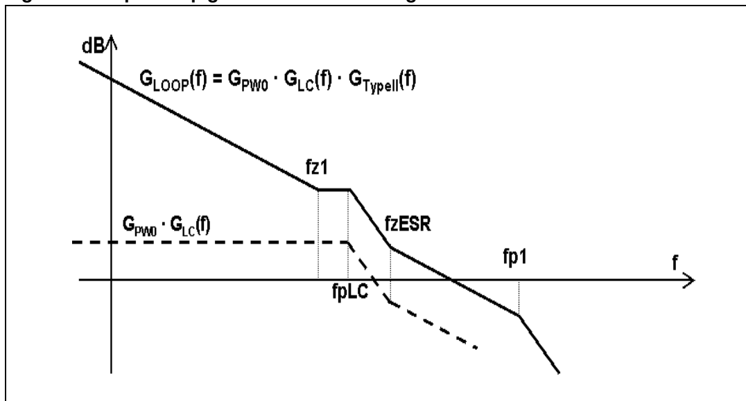
Figure 13. Open-loop gain: module Bode diagram
