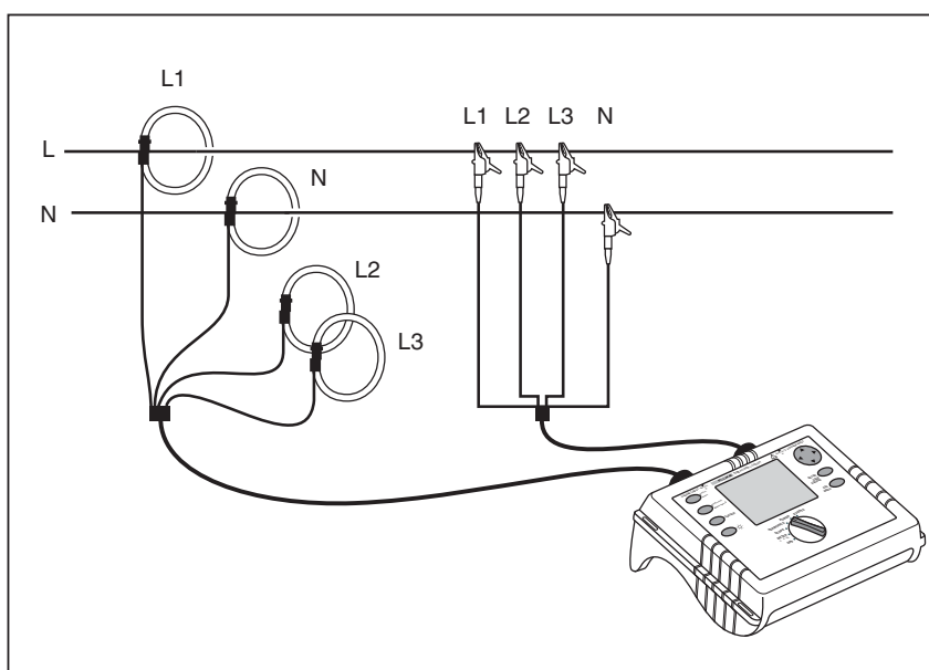
Figure 5. Single Phase Connections
