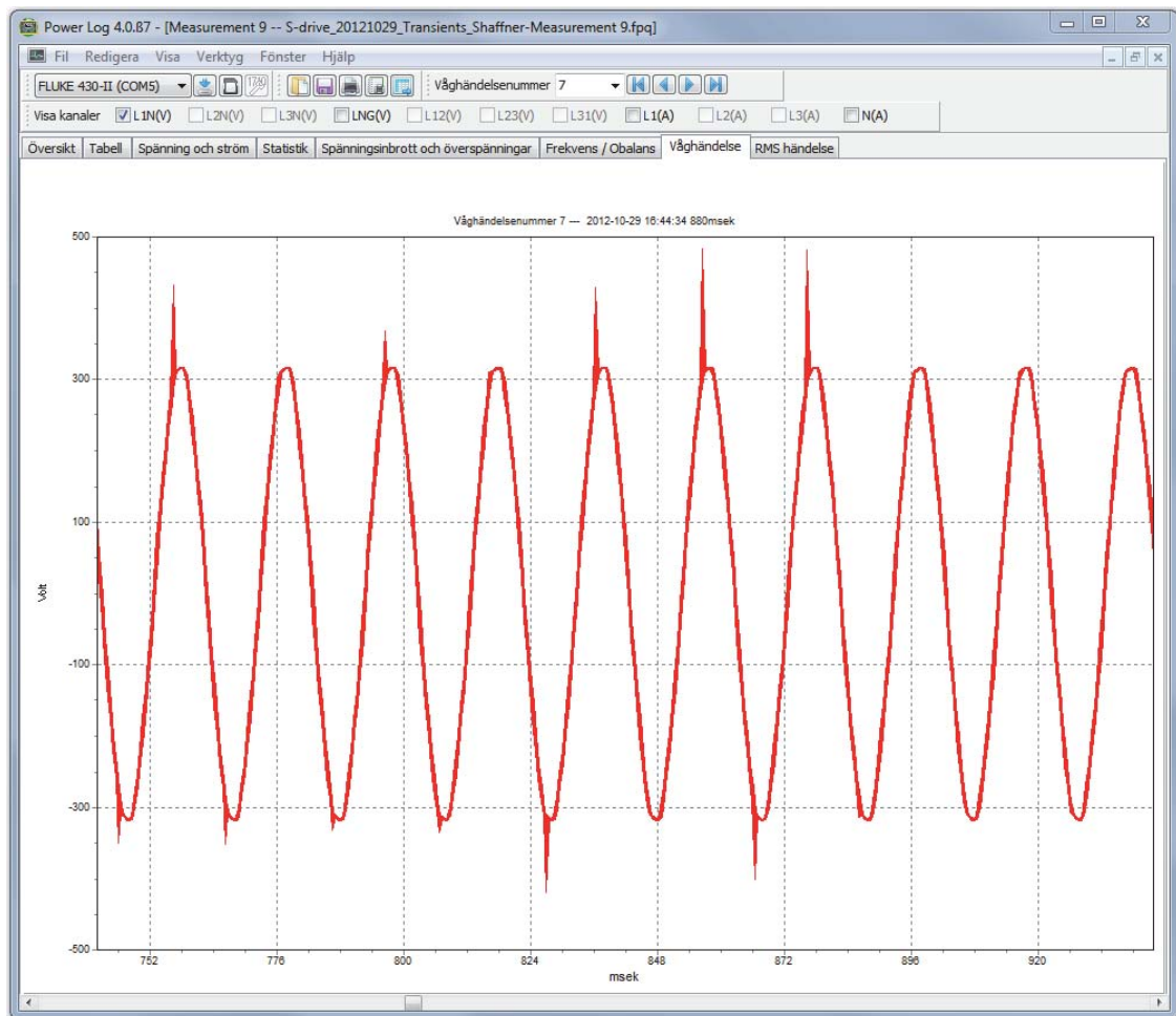
Figur 12. Transient vågform
