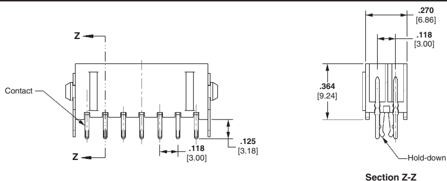
Section Z-Z
